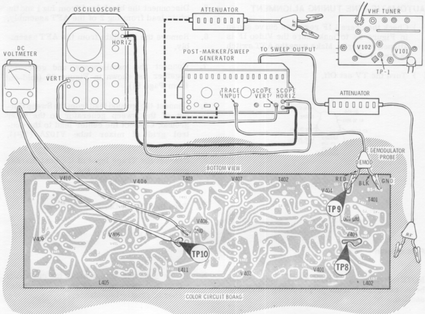
Figure 20 COLOR AND BANDPASS ALIGNMENT
