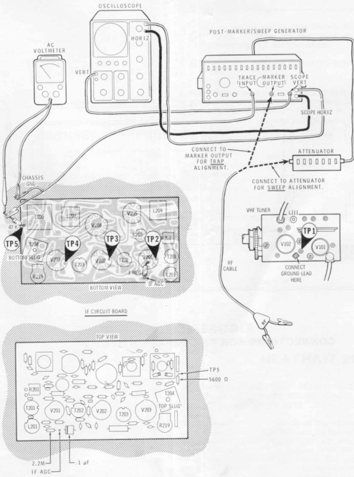
FIGURE 19 SWEEP ALIGNMENT
