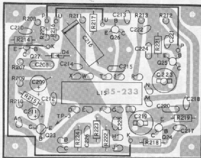
SWEEP CIRCUIT BOARD (VIEWED FROM FOIL SIDE)
