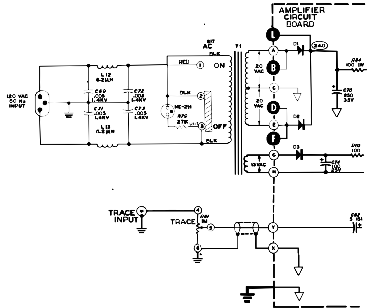
SCHEMATIC OF THE HEATHKIT® TV POST-MARKER/SWEEP GENERATOR MODEL IG-57A
