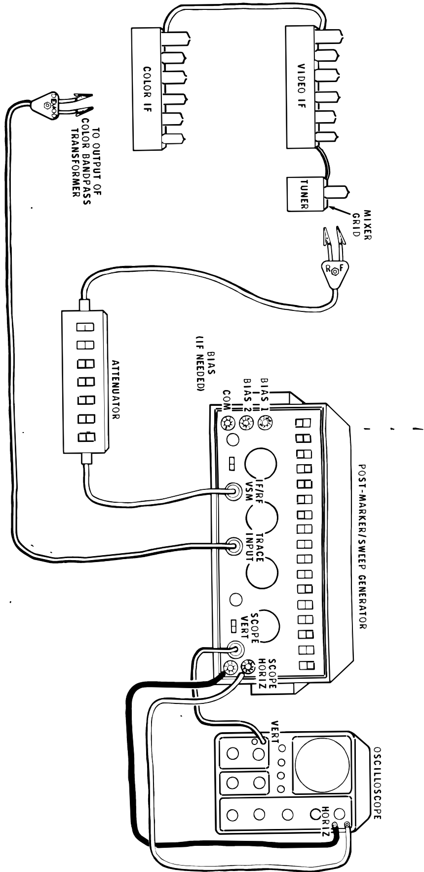
FIGURE 14 CONNECTIONS FOR IF-VSM ALIGNMENT
