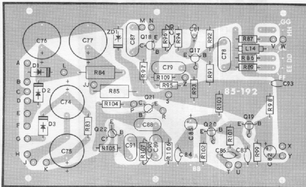
AMPLIFIER CIRCUIT BOARD (VIEWED FROM FOIL SIDE)
